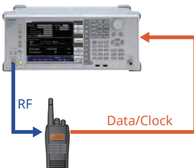
Rx Sensitivity Test Setup
